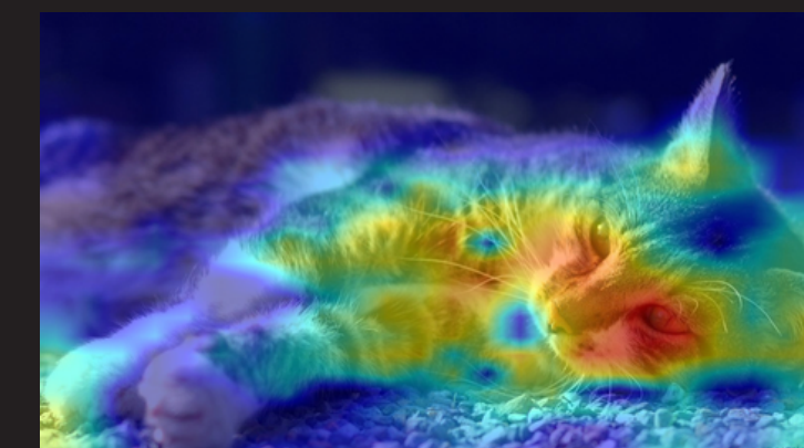
Grad-CAM
